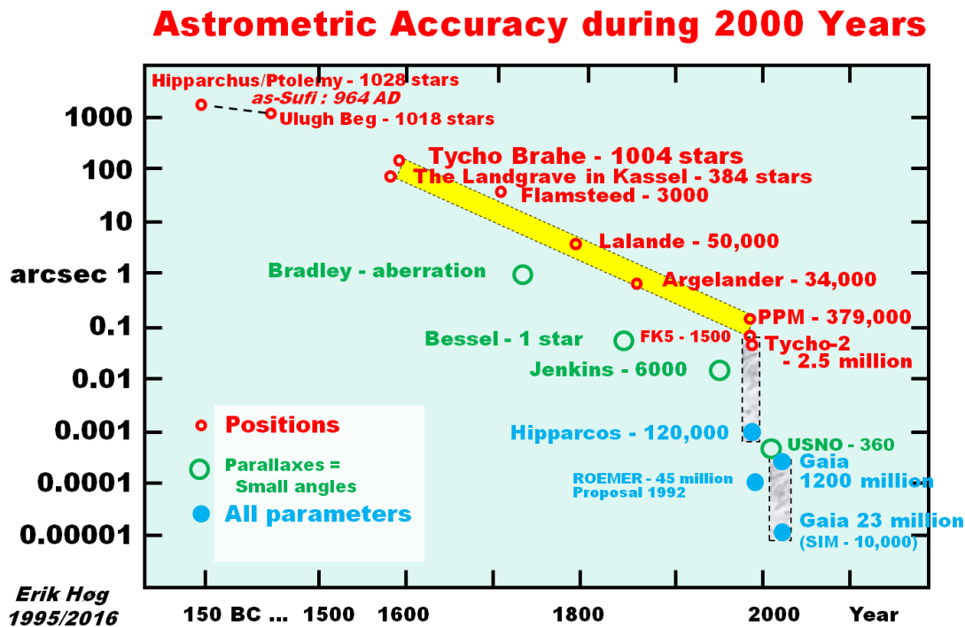
Fig. 1a. Astrometric accuracy during 2000 years: Høg-2016. The accuracy was greatly improved shortly before 1600 AD by the Landgrave in Kassel and by Tycho Brahe in Denmark. The following 400 years brought even larger but much more gradual improvement before space techniques with the Hipparcos satellite started a new era of astrometry.
