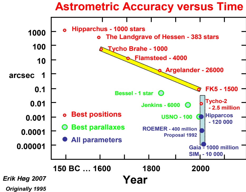
Figure 3. Astrometric accuracy through 22 centuries from Hipparchus to Gaia.
