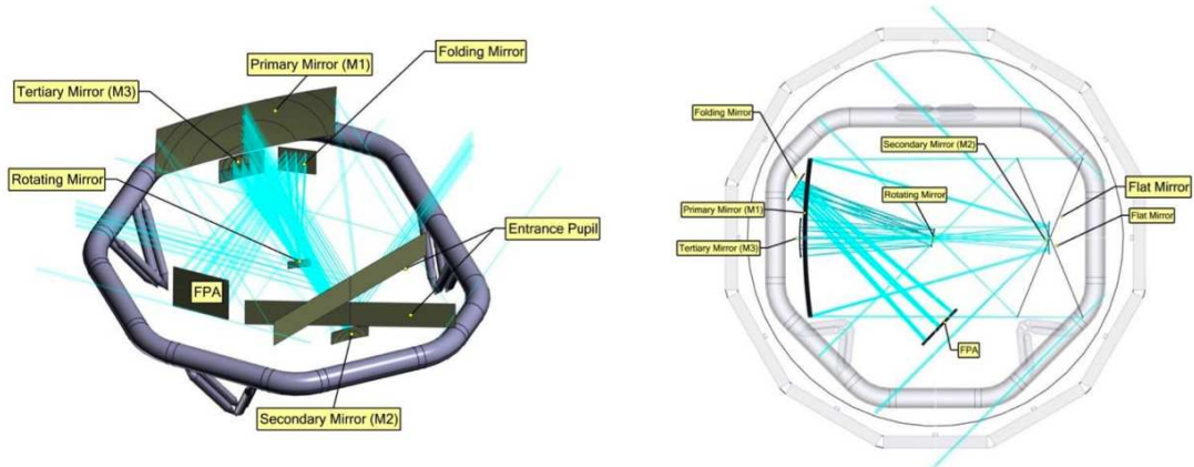
Figure 1: GaiaNIR optical surfaces and the light path (left) and Top view of the GaiaNIR Light path (right). Images from the ESA CDF study report.
